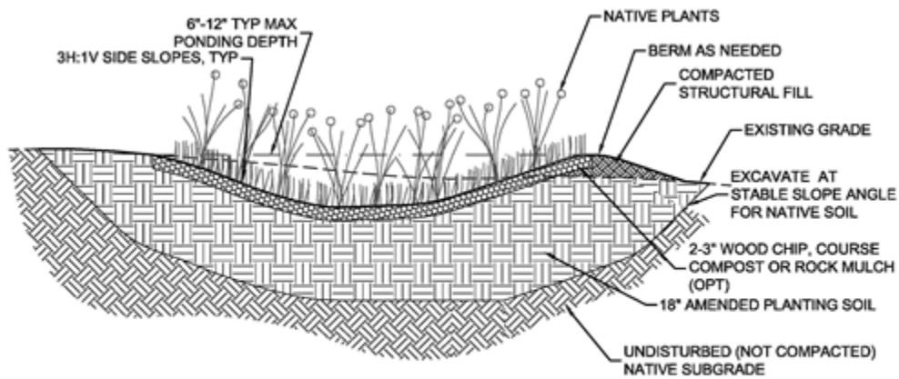
LID 1.06 Infiltration Rain Garden with Planting Soil NTS
